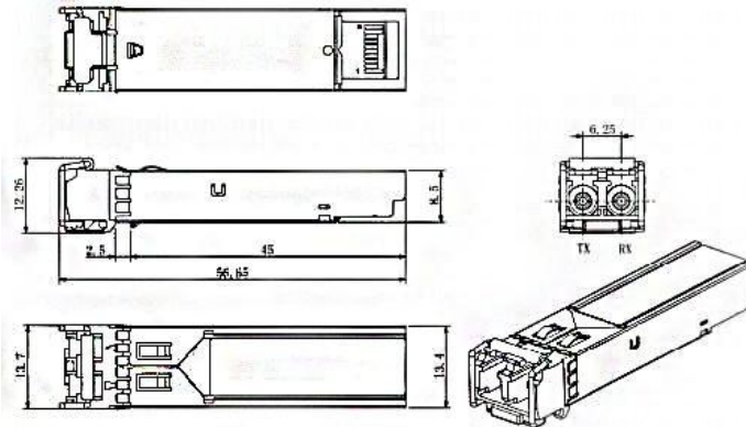
Figure 6. Mechanical Drawing
