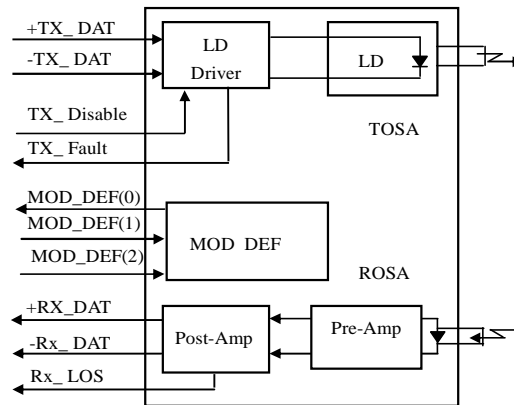
Figure1: Block Diagram
