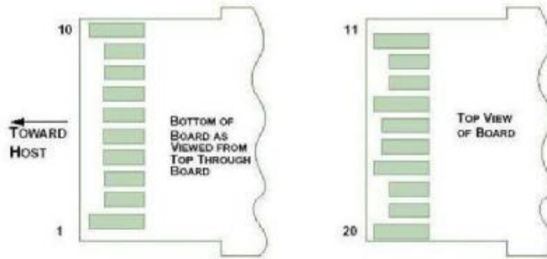
Figure 4: Pin Definitions
